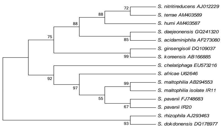
Figure 5 Hypothesis of 16s-rRNA gene based phylogenetic relationships of S. maltophilia IR11 and S. pavanii IR20 to members of the genus Stenotrophomonas constructed by (A) maximum parsimony (B) maximum likelihood and (C) neighbor-joining methods. Bootstrap values are shown at the nodes.
